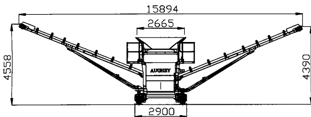
Operating end view
