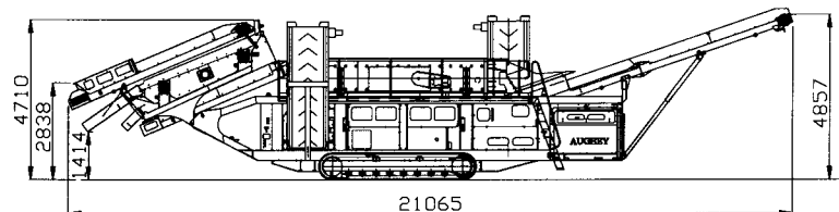
Operating side view
