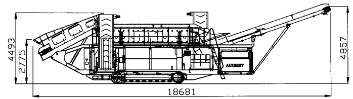
Operating side view
